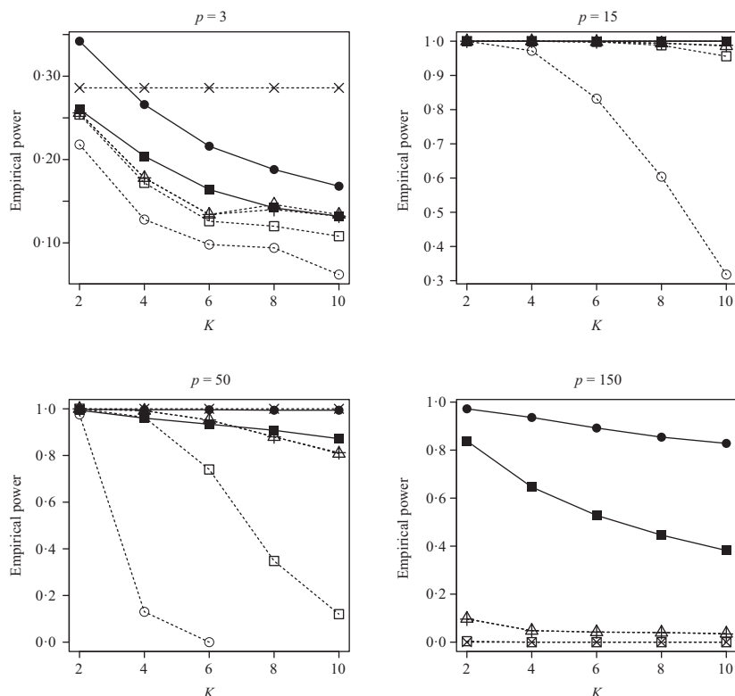
Fig. 1. Plots of empirical power against lag K for the new tests T_n (solid and ■ lines) and T_n^* (solid and ● lines), the portmanteau tests Q_1 (dashed and △ lines), Q_2 (dashed and + lines) and Q_3 (dashed and □ lines), the Lagrange multiplier test (dashed and ○ lines), and Tiao and Box's test (dashed and ×). The data are generated from Model 4 with sample size n = 300 . The nominal level is \alpha = 5\% .
